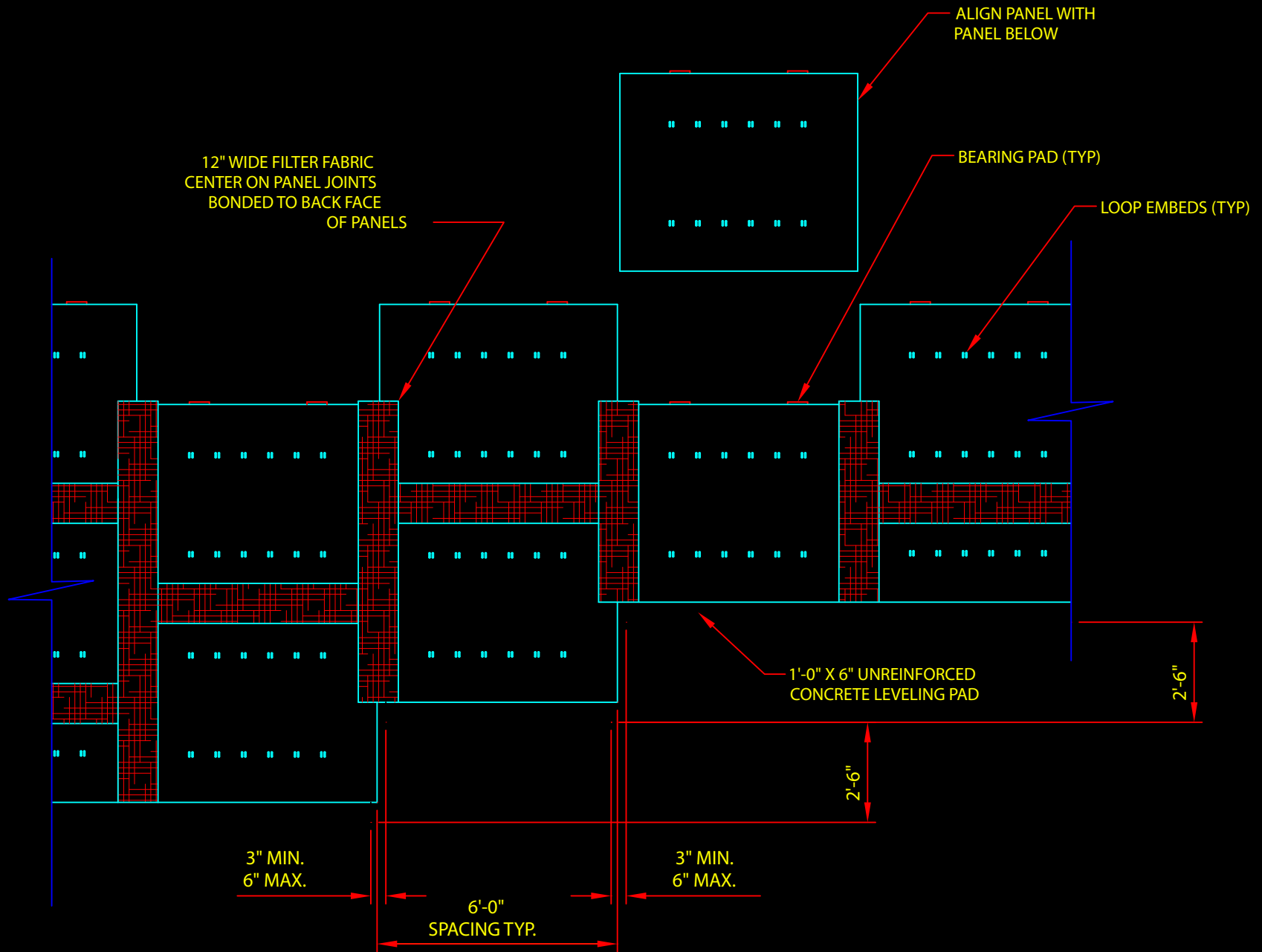
STEPPING OF LEVELING PAD WITH 5X6 PANELS
